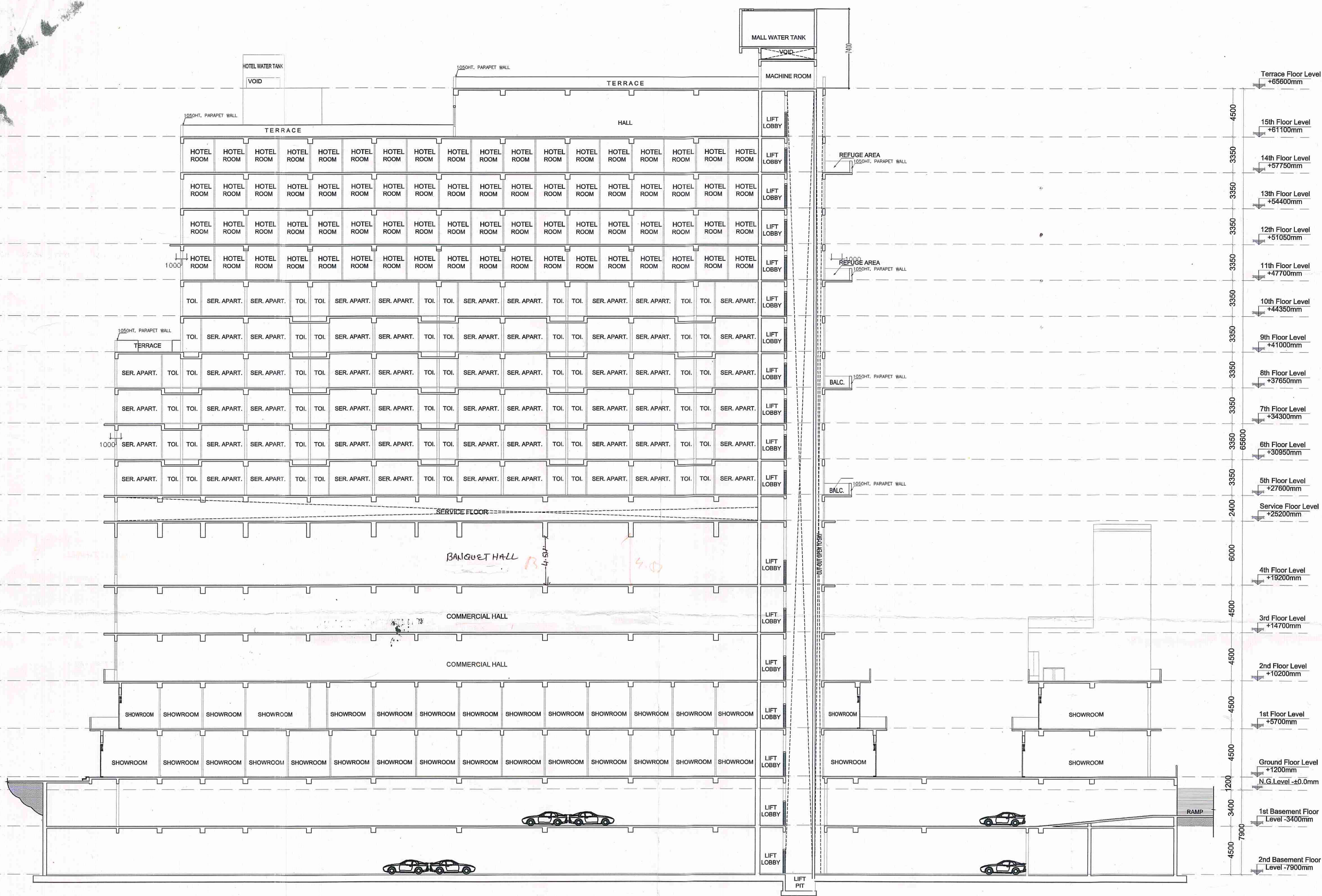
SECTION C-C
